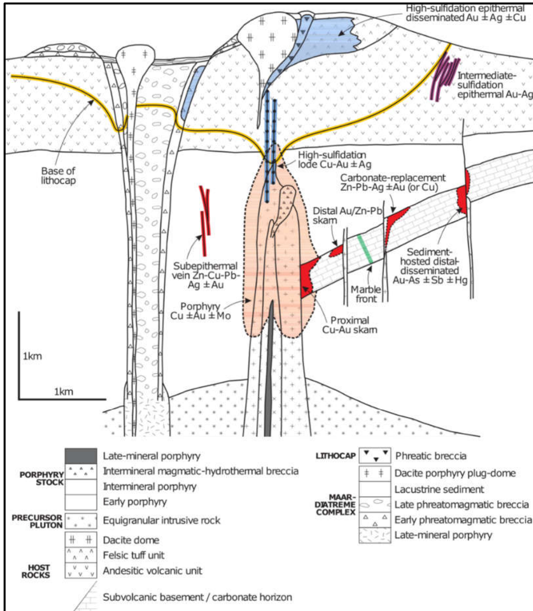
Figure 10: Deposit Model
