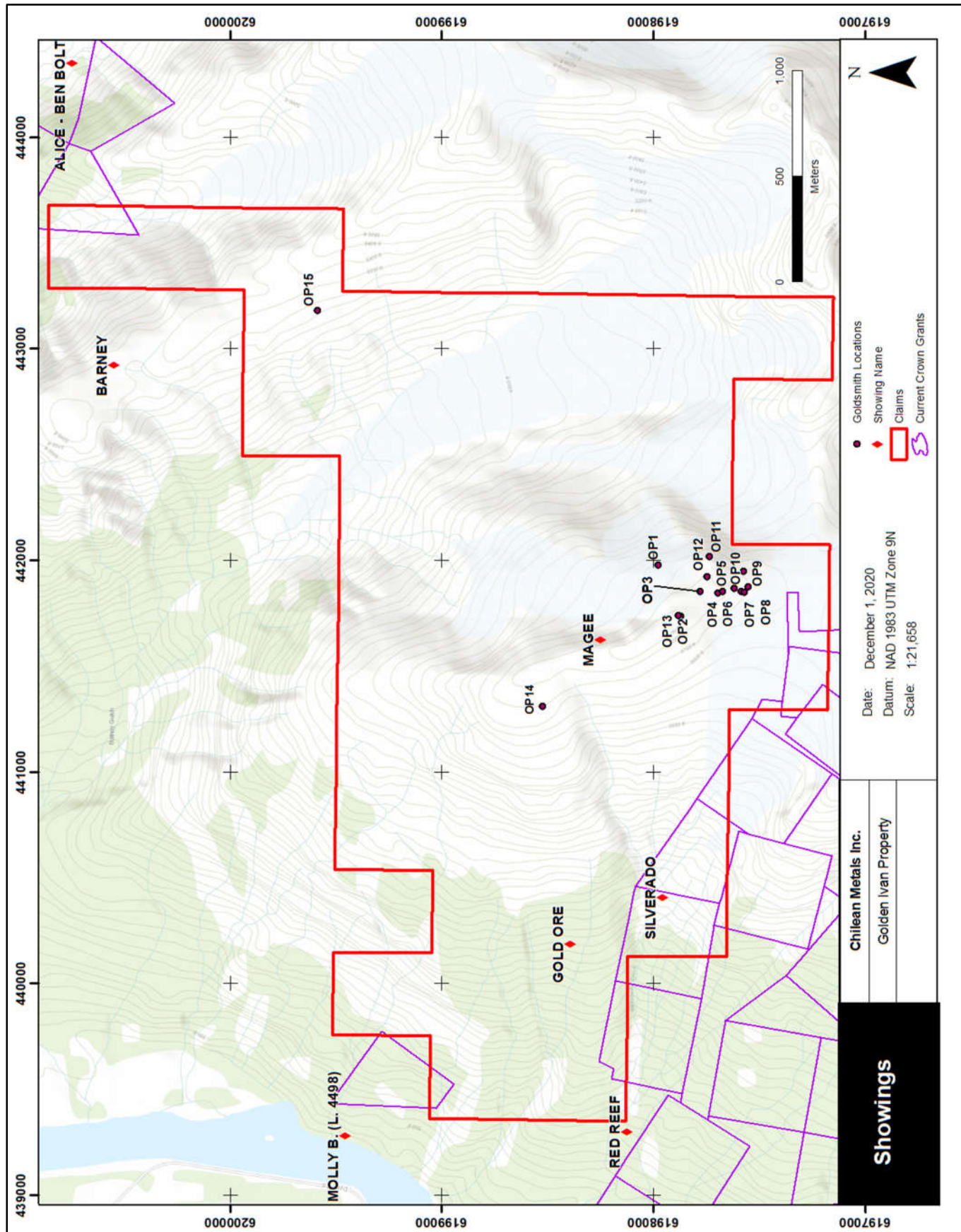
Figure 9: Minfile Showings
