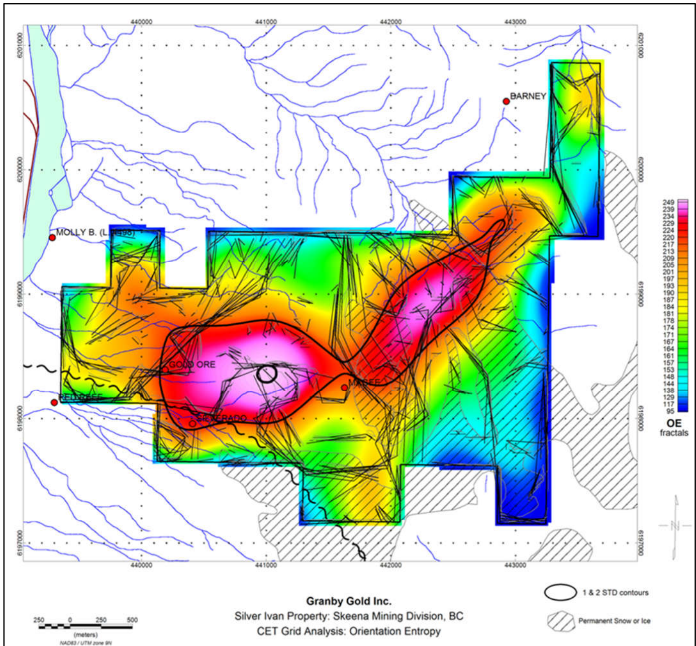
Figure 5: CET Grid Analysis: Orientation Entropy w/ 1 and 2 STDs above mean
