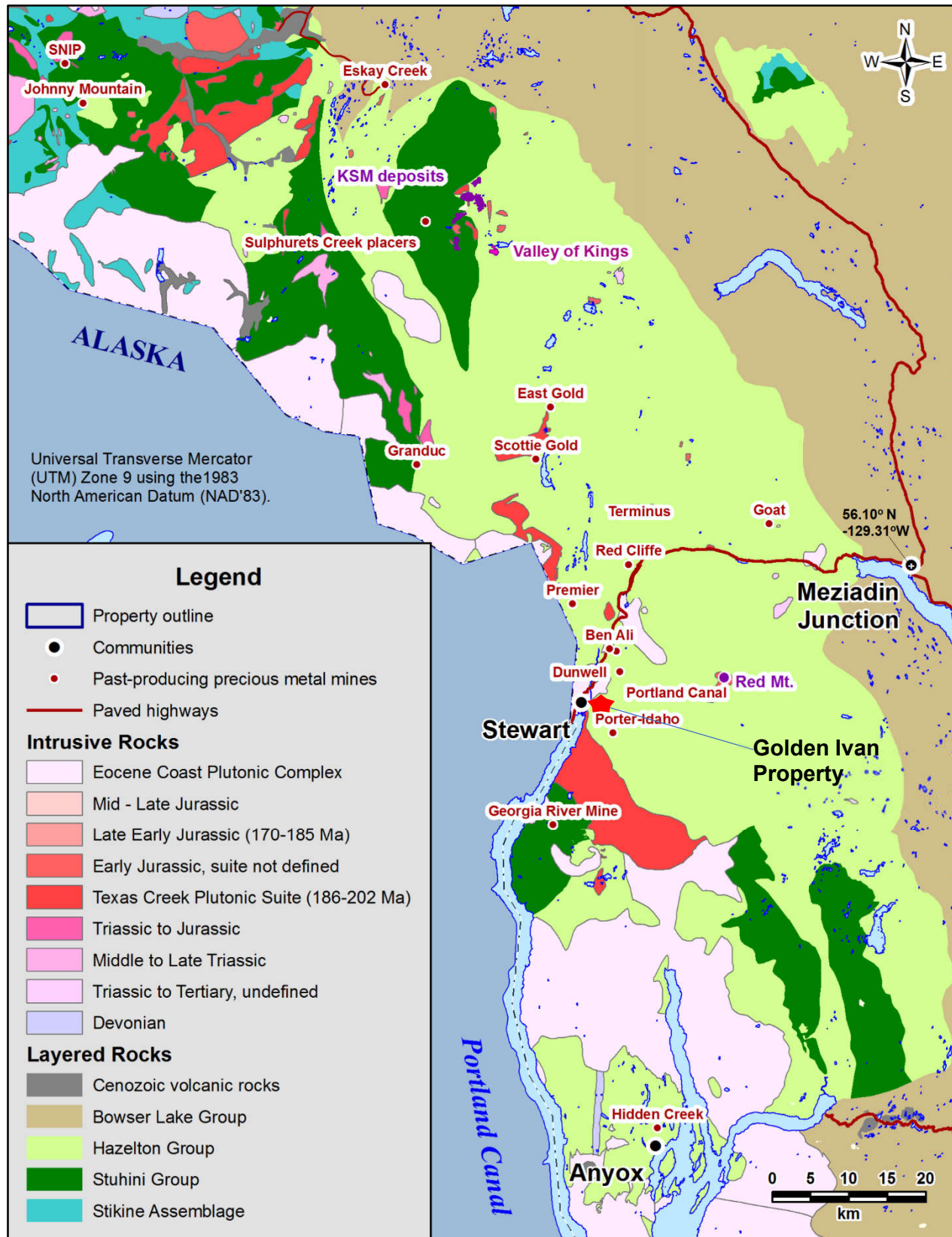
Figure 7: Regional Geology
